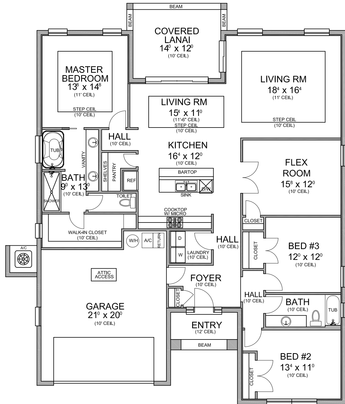
FLOOR PLAN
